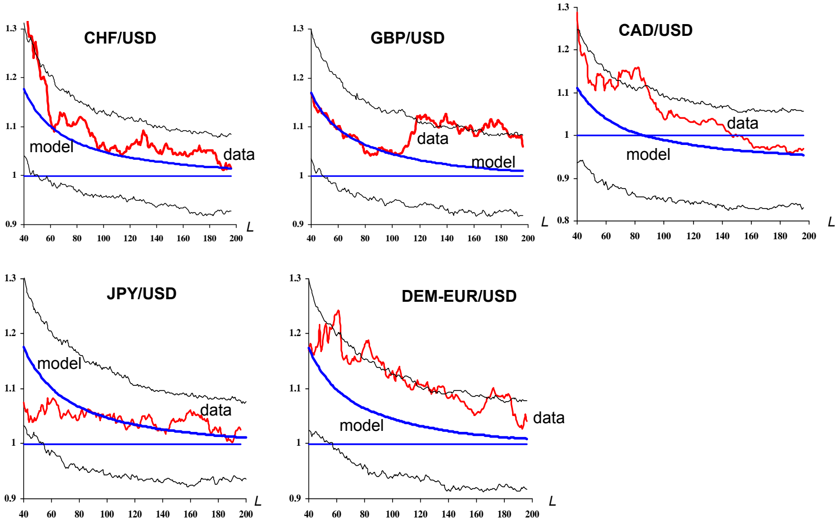
Figure 5 Out-of-Sample Fit Model versus Data: MSE^{Model}/MSE^{RW*}
